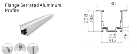
Bendable Serrated Aluminum Profile
