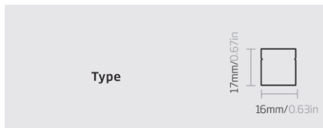
Aluminum Profile
